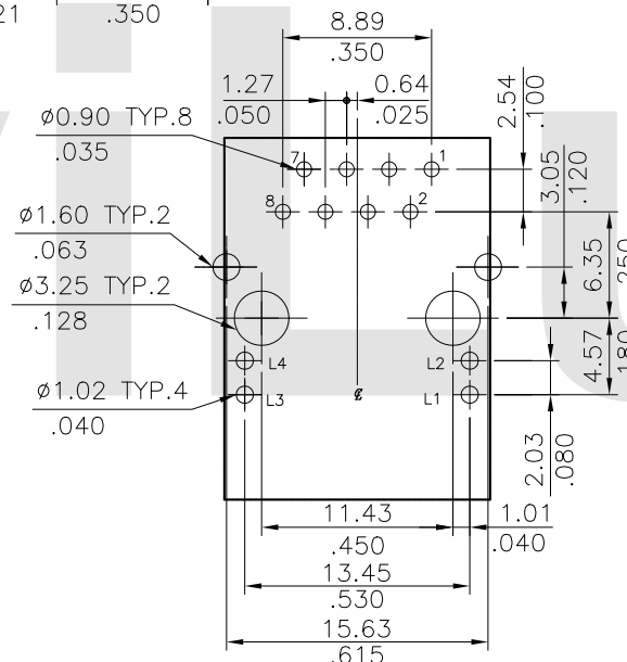
Recommended P.C. Board Layout (TOP VIEW) Tolerances: ±0.05/.002
