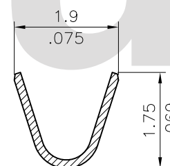
SEC. B-B SCALE 10/1
