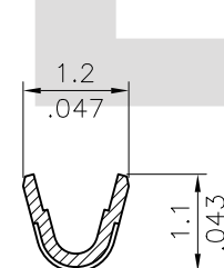
SEC. A-A SCALE 10/1
