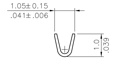
SEC.:B-B
