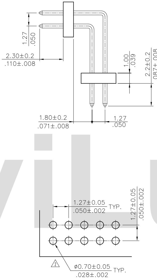
Recommended P.C. Boarded Layout
