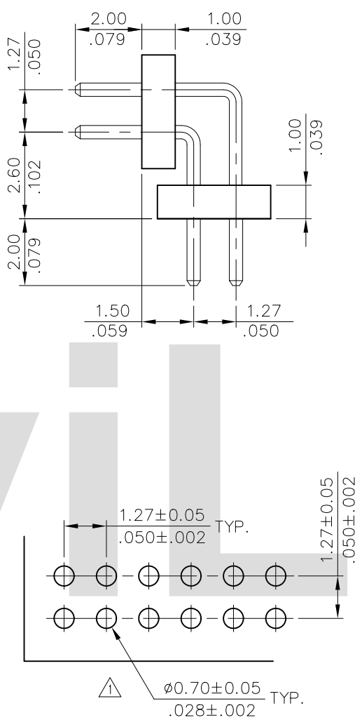
Recommended P.C. Boarded Layout
