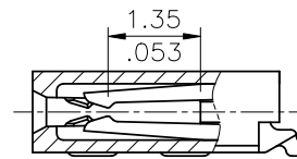
SEC.: X-X
