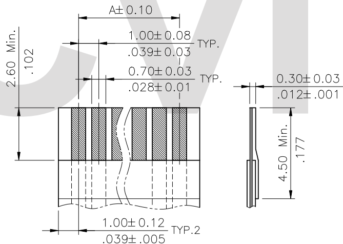
Accommodated FFC
