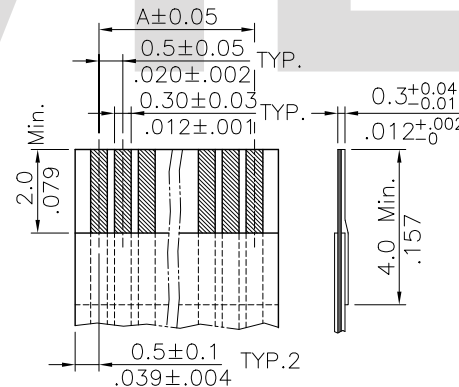
Accommodated FFC/FPC
