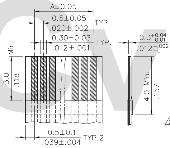
Accommodated FFC/FPC
