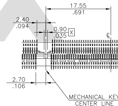
TYPE 2 POWER SUPPLY 1.8 V (CS702002A00)
