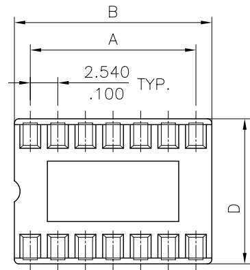
Typical 24,28,32,40 Circuits
