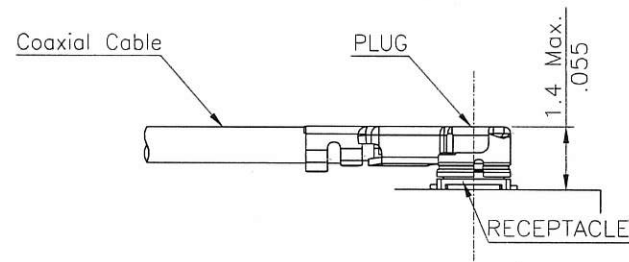
Mating Height
