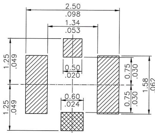
Recommended P.C. Board Layout (TOLERANCE: \pm 0.05 )
