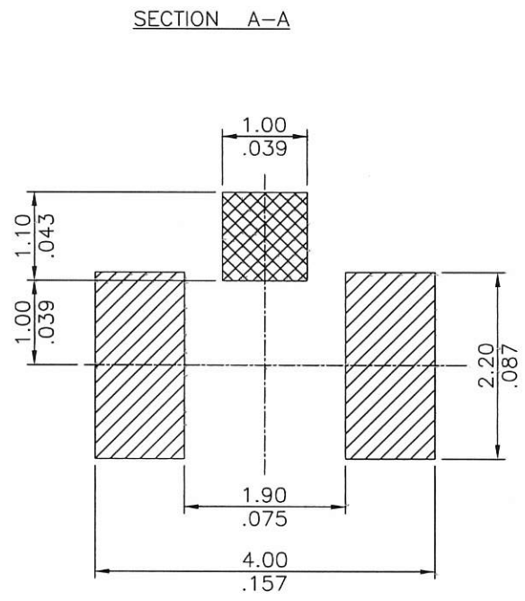
Recommended P.C. Board Layout (TOLERANCE: ±0.05)
