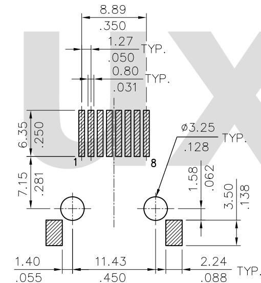
Solder Pad Pattern
