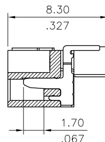
SEC. E-E
