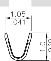
SEC. A-A SCALE 10/1
