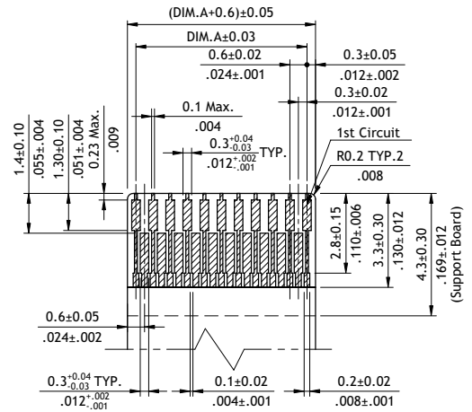
Recommended FPC Dimension (Thickness: 0.2±0.03mm)
