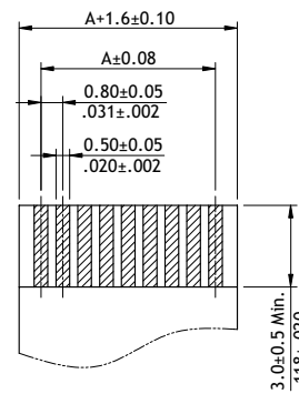
Accommodated FFC/FPC
