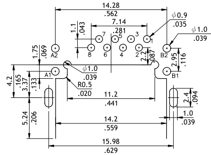
Recommended P.C. Board Layout Tolerance: ±0.05mm
