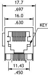
8 Positions
