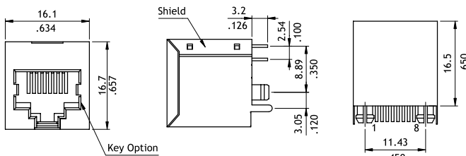
Bottom View
