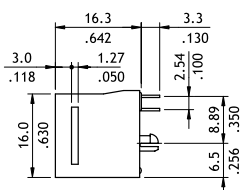
6 Positions
