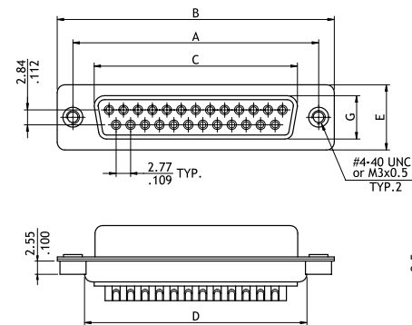
Receptacle Connector (K0/K1 Type)
