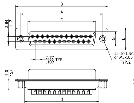
Receptacle Connector (K0/K1 Type)
