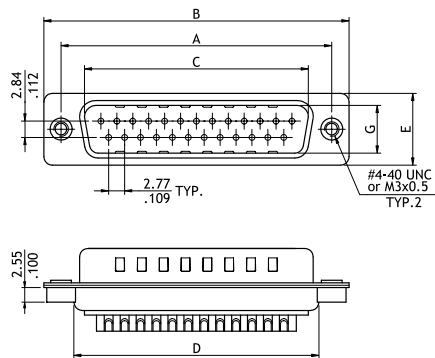
Plug Connector (K0/K1 Type)
