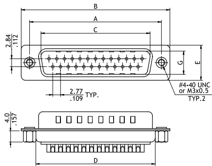
Plug Connector (K0/K1 Type)
