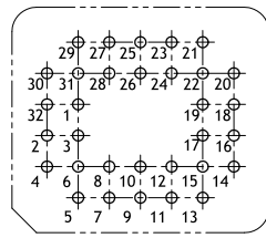
P. C. Board Hole Pattern
