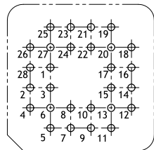
P. C. Board Hole Pattern
