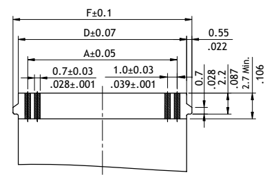
Accommodated FFC/FPC (TYPE2)
