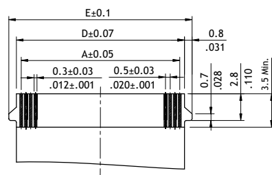
Accommodated FFC/FPC (TYPE1)
