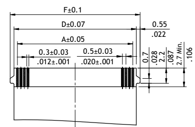
Accommodated FFC/FPC (TYPE2)
