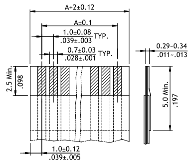
Accommodated FFC/FPC
