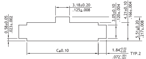
Panel Cutout Size
