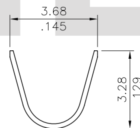
SEC.: C-C
