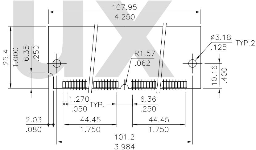
Module P.C. Board Layout
