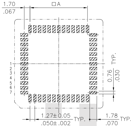
Solder Pad Pattern
