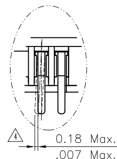
Detail "B"
