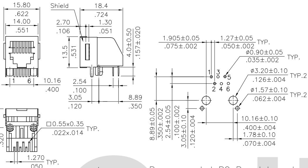
6P6C/6P4C Recommended PC Board Layout
